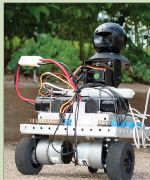
A sample TeRK you'll build in Foothill's ENGR 20 class.
